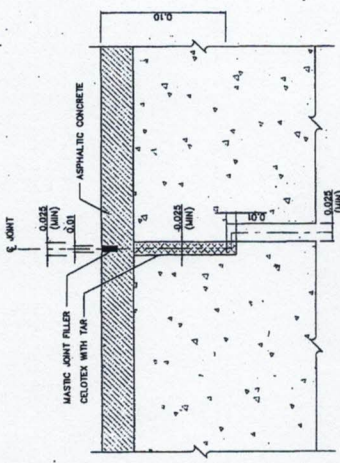
(MAXIMUM GAP 40 MM.) TYPICAL SECTION OF SMALL MOVEMENT NOT TO SCALE
