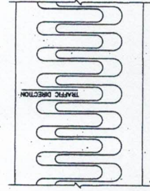
PLAN OF FINGER JOINT
