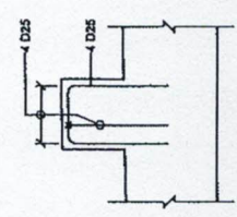
1 DETAIL SCALE 1:20
