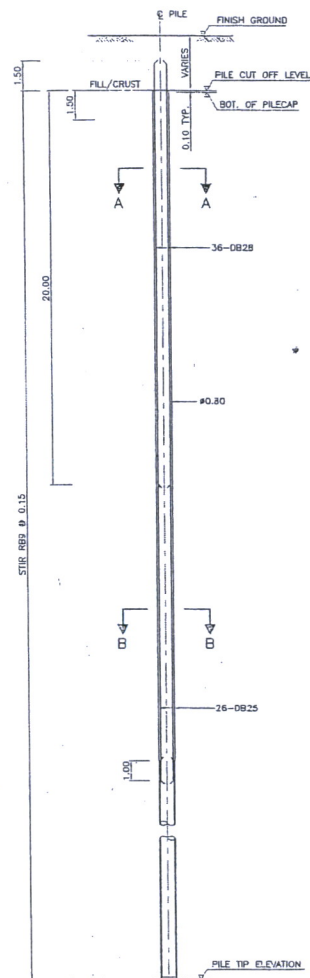
BORED PILE, \phi 0.80 M. SCALE 1 : 125
