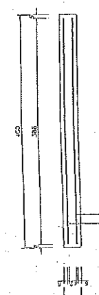
SECTION B-B BEARING TYPE "FR"
